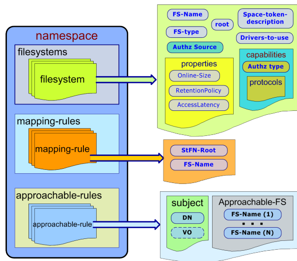
Figure 2: Namespace structure
